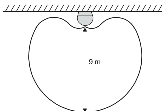
glass break detector working range diagram
